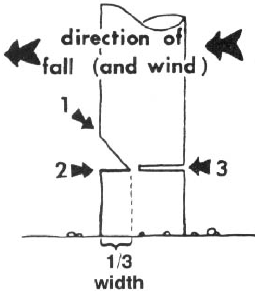
Chainsaw felling; note sequence of cuts.
