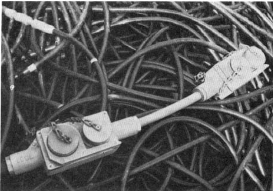
Seismic cable. Note cableheads.
